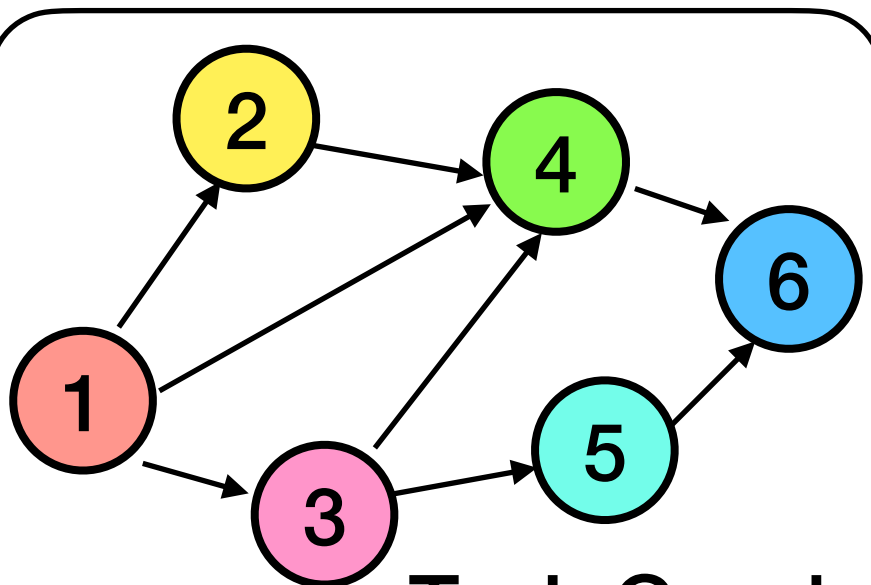
Task Graph
